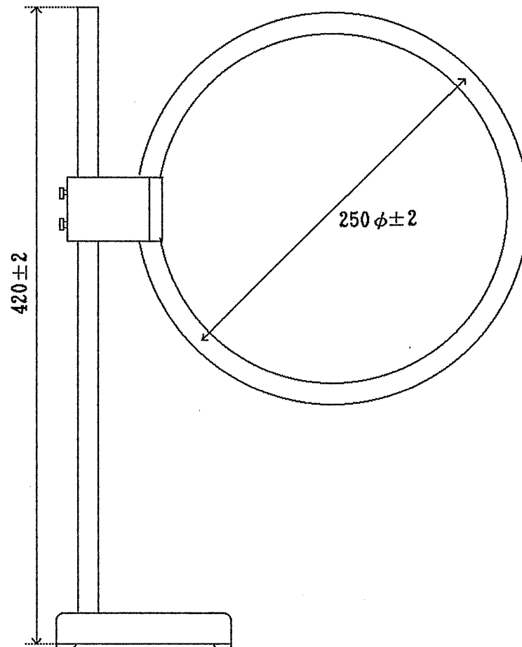
Figure 9-1. Outline drawing
