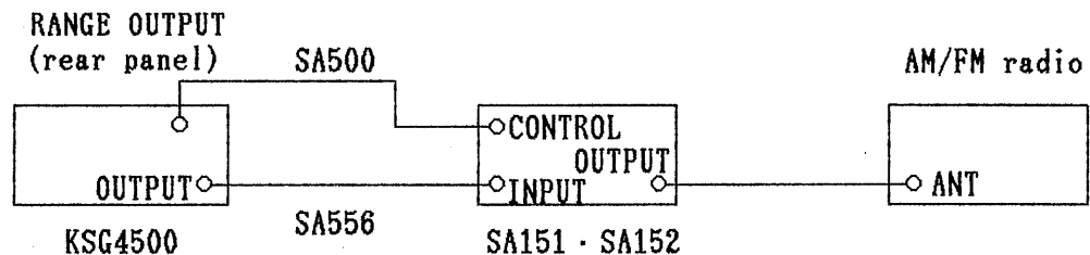
Figure 9-5. Connection Example
